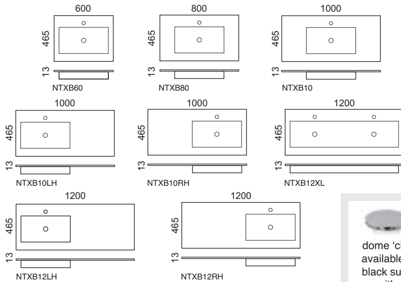
NTXB12RH NTX 1200 basin RH (w)1200 x (d)465 x (h)13mm 1 tap hole basin - right hand slate - cement
